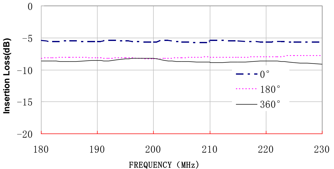
Insertion Loss, Major States only
