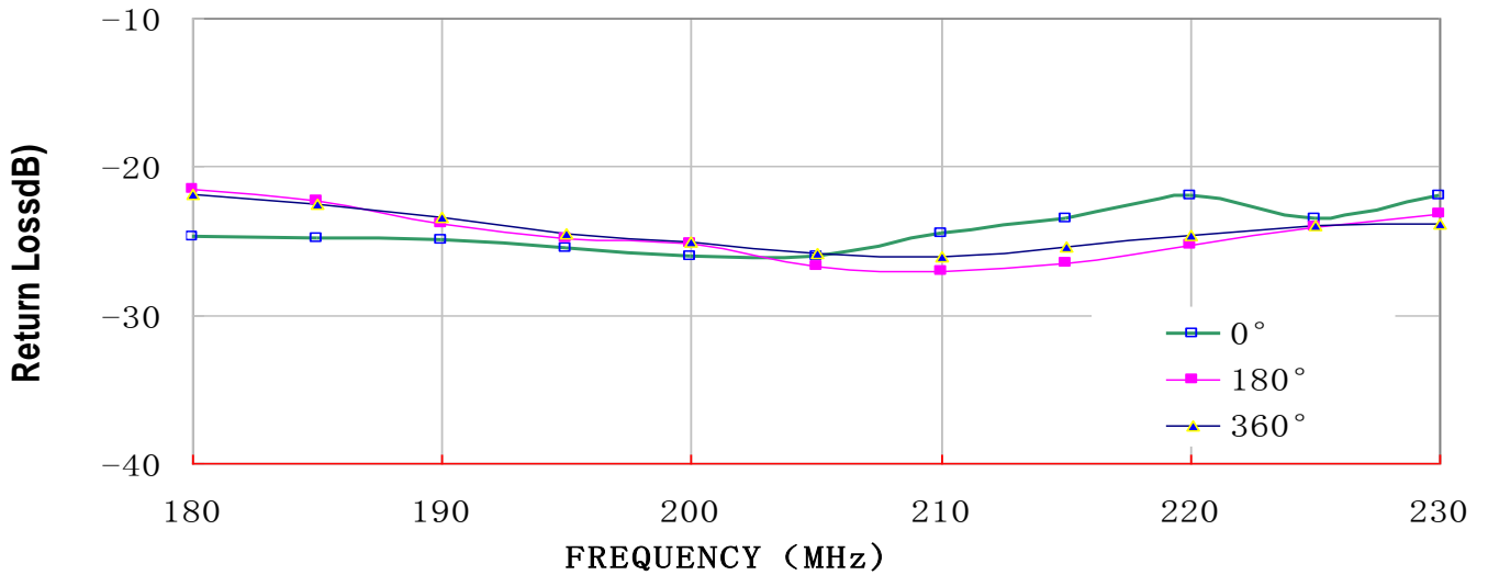
Return Loss, Major States Only
